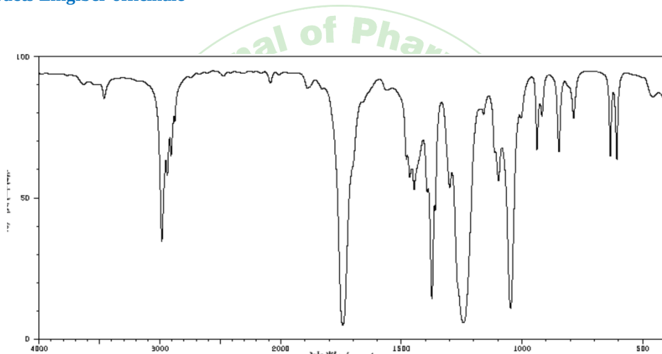
Figure: 4 FTIR Spectrum of Zingiber officinale Extract
